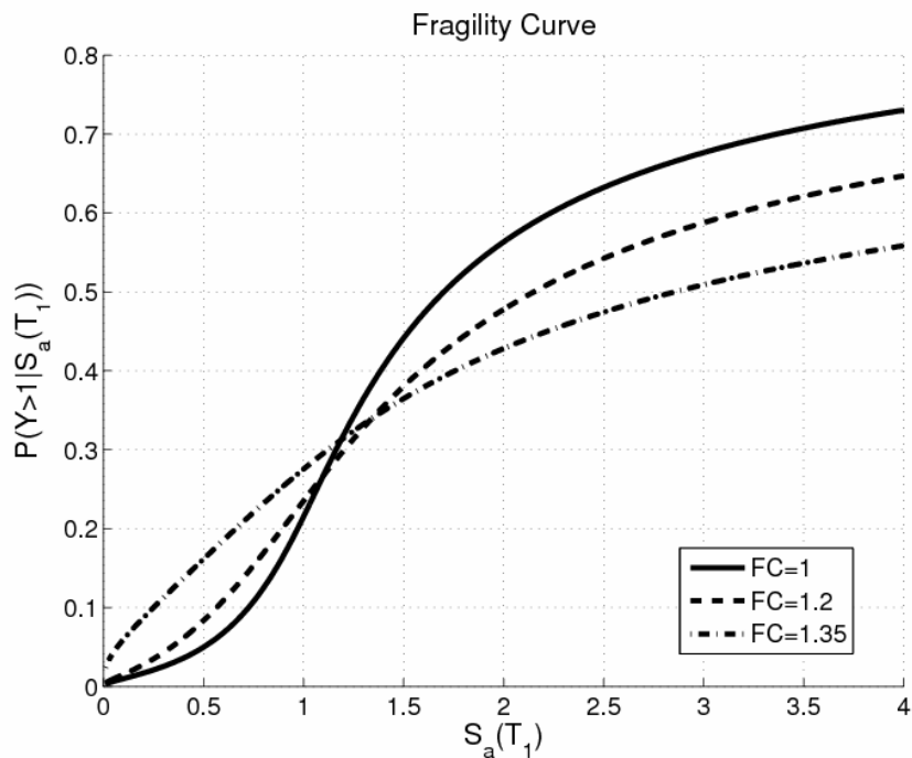
Figure 6. The Fragility curves corresponding to each CF value, the code-compatible dynamic method.
